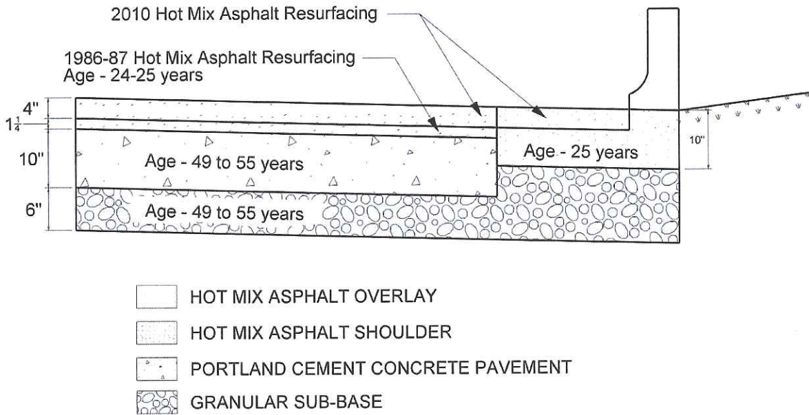
Figure 1-12 - I-290 Pavement Construction History through 2010
