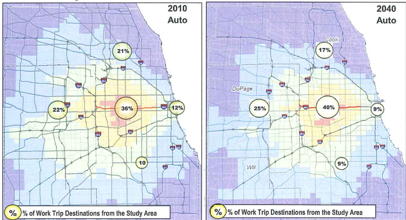
Figure 1-6 - 2010 & 2040 AM Peak Period Auto Travel Time Contours
